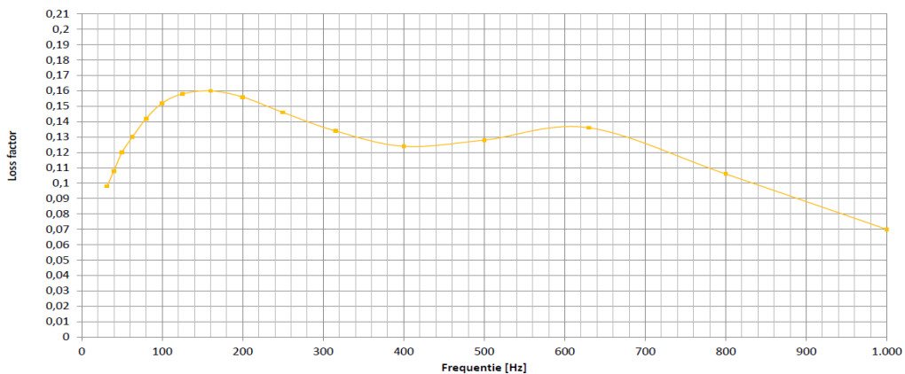
Damping HexaNaval AL 0,5 on 5 mm aluminium
